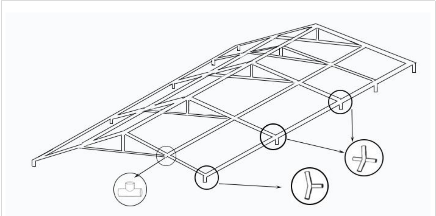
Connect reinforced bars together with bungee balls.
