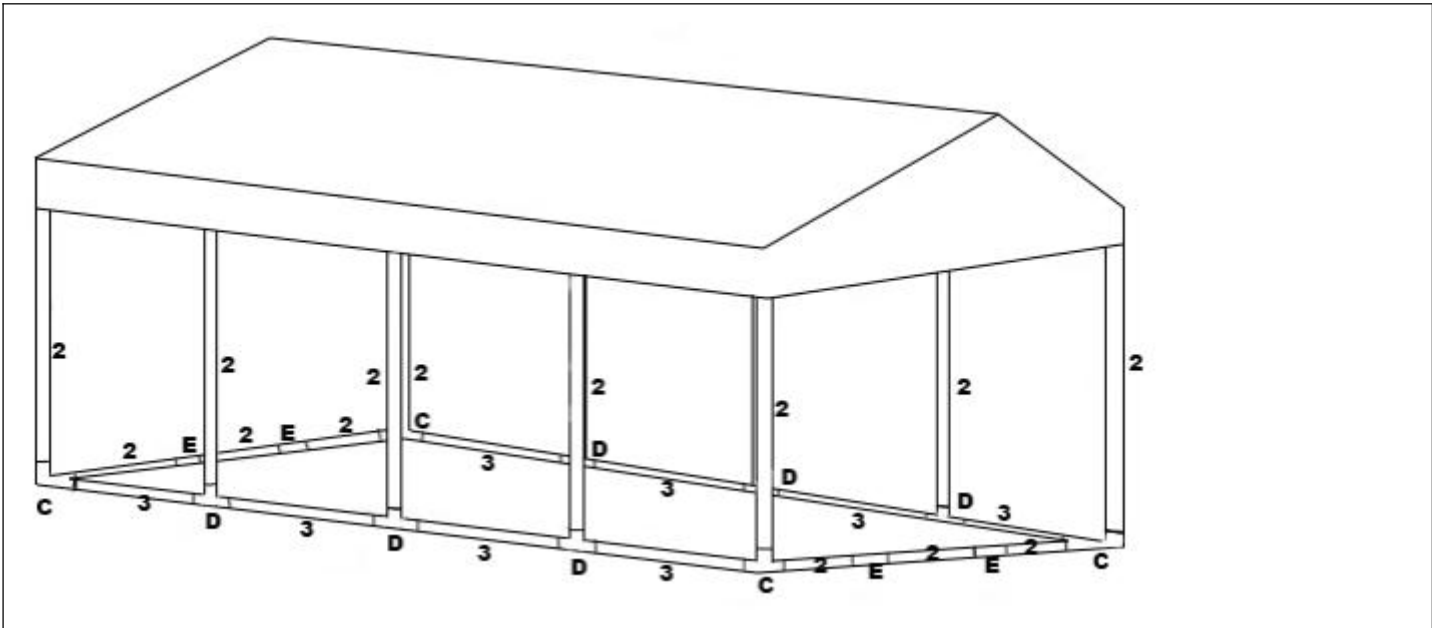
4. Insert leg tubes and connect the legs with ground bars.
